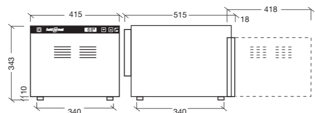
Hold-o-mat (Household) (Power consumption: 1 kW) - Capacity: 3 x 2/3 65 mm or 2 x 2/3 100 mm containers - Weight: 21 kg
