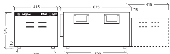
Hold-o-mat small (Power consumption: 1 kW) Hold-o-mat small with internal temperature gauge (Power consumption: 1 kW) - Capacity: 3 x 1/1 65 mm or 2 x 1/1 100 mm containers - Weight: 24 kg
