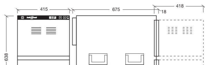
Hold-o-mat «big model» (Power consumption: 1.8 kW) - Capacity: 7 x 1/1 65 mm or 4 x 1/1 100 mm containers - Weight: 38 kg
